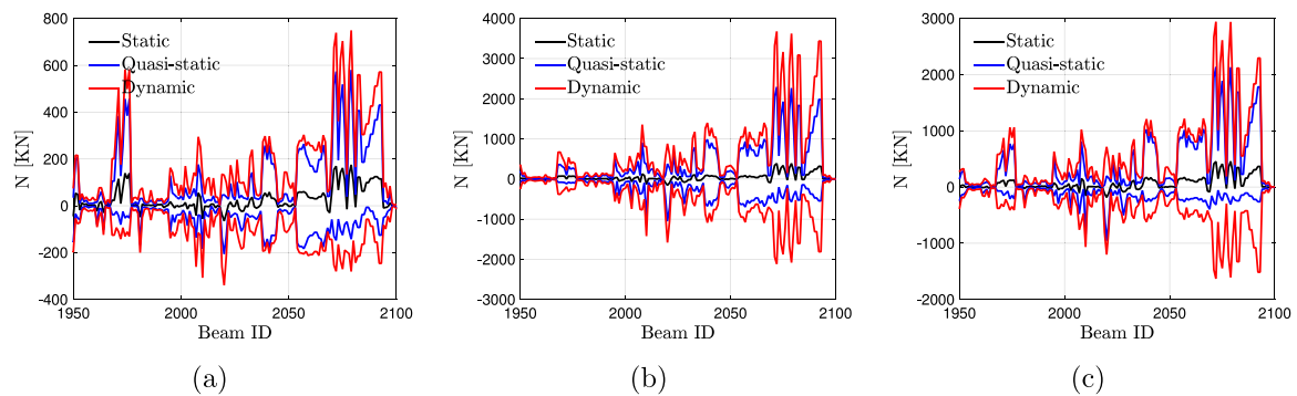
Fig. 20. Comparison between design envelopes for axial forces obtained from the static, quasi-static and dynamic components of the structure response: (a) 0°, (b) 60° and (c) 120°.
