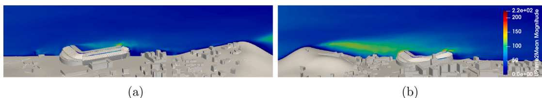
Fig. 8. Flow visualization of the wind coming from different terrains, coloured by (|U'|/|U|)^2 : (a) 30° and (b) 210°.
