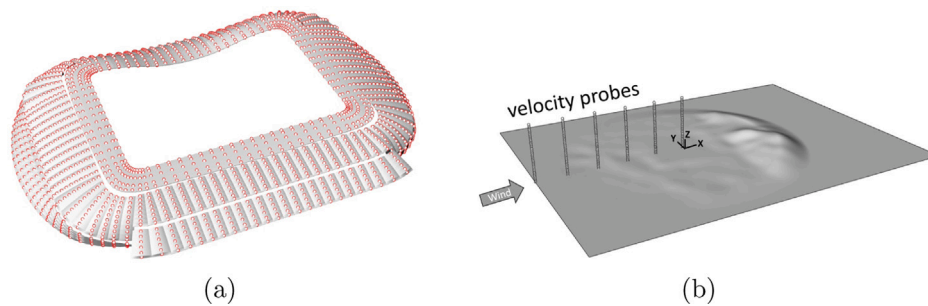
Fig. 4. The distribution of the pressure probes on the stadium roof (a) and the velocity probes in the empty domain (b).
