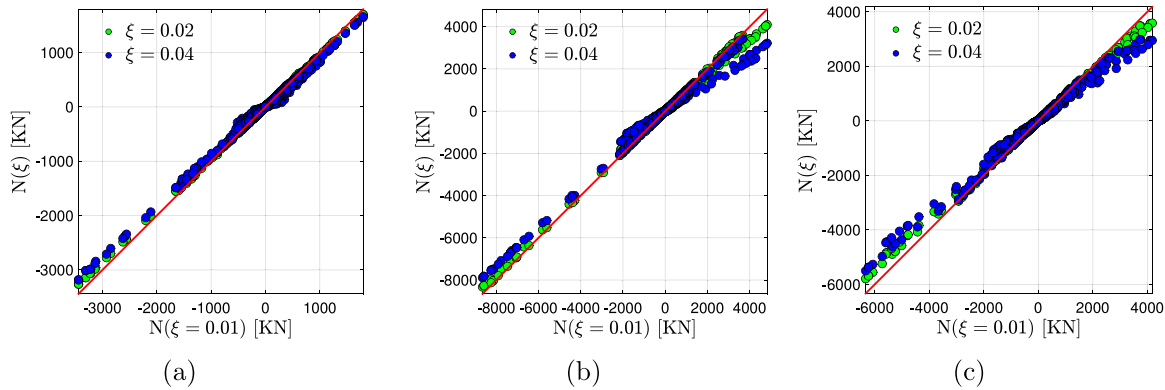
Fig. 18. Comparison between extreme axial forces obtained with different damping ratios: (a) 0°, (b) 60° and (c) 120°.
