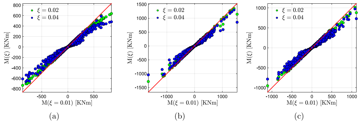
Fig. 19. Comparison between extreme bending moments obtained with different damping ratios: (a) 0°, (b) 60° and (c) 120°.
