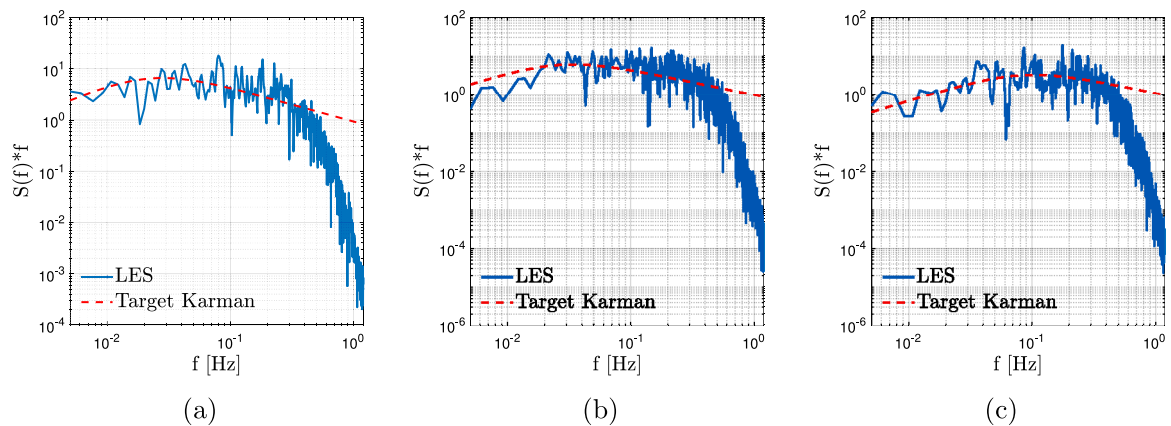
Fig. 6. Spectra of the velocity components measured at H_z : along-wind component (a), cross-wind component (b) and vertical component (c).
