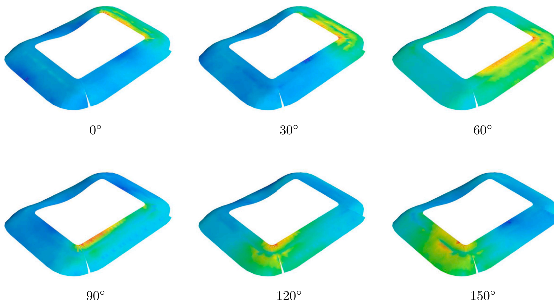
Fig. 9. Proper Orthogonal Decomposition, an overview of the first mode for angles up to 150° (colorbar not reported as the POD modes are not defined in amplitude). (For interpretation of the references to colour in this figure legend, the reader is referred to the web version of this article.)
