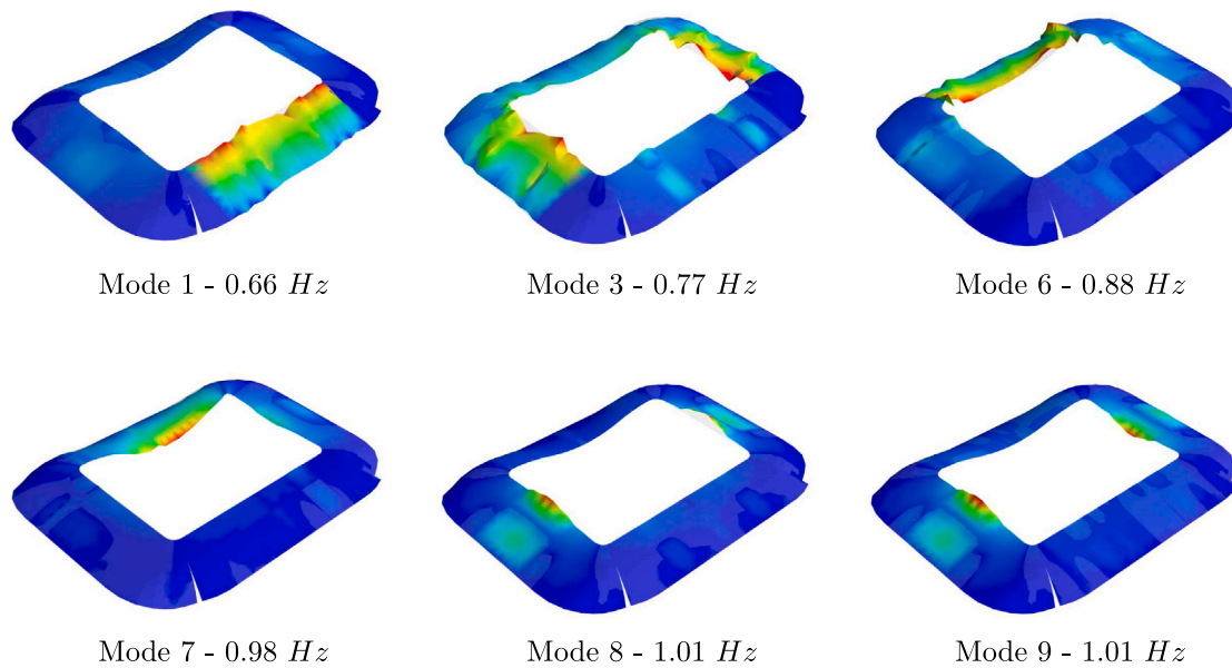
Fig. 14. Overview of the first ten structural modes, only those potentially relevant to wind loading are reported (colorbar not reported as the structural modes are not defined in amplitude). (For interpretation of the references to colour in this figure legend, the reader is referred to the web version of this article.)
