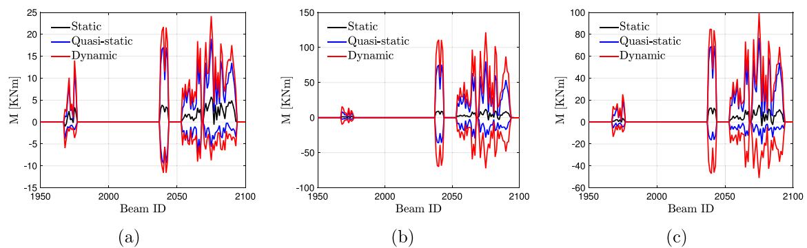
Fig. 21. Comparison between design envelopes for bending moments obtained from the static, quasi-static and dynamic components of the structure response: (a) 0°, (b) 60° and (c) 120°.
