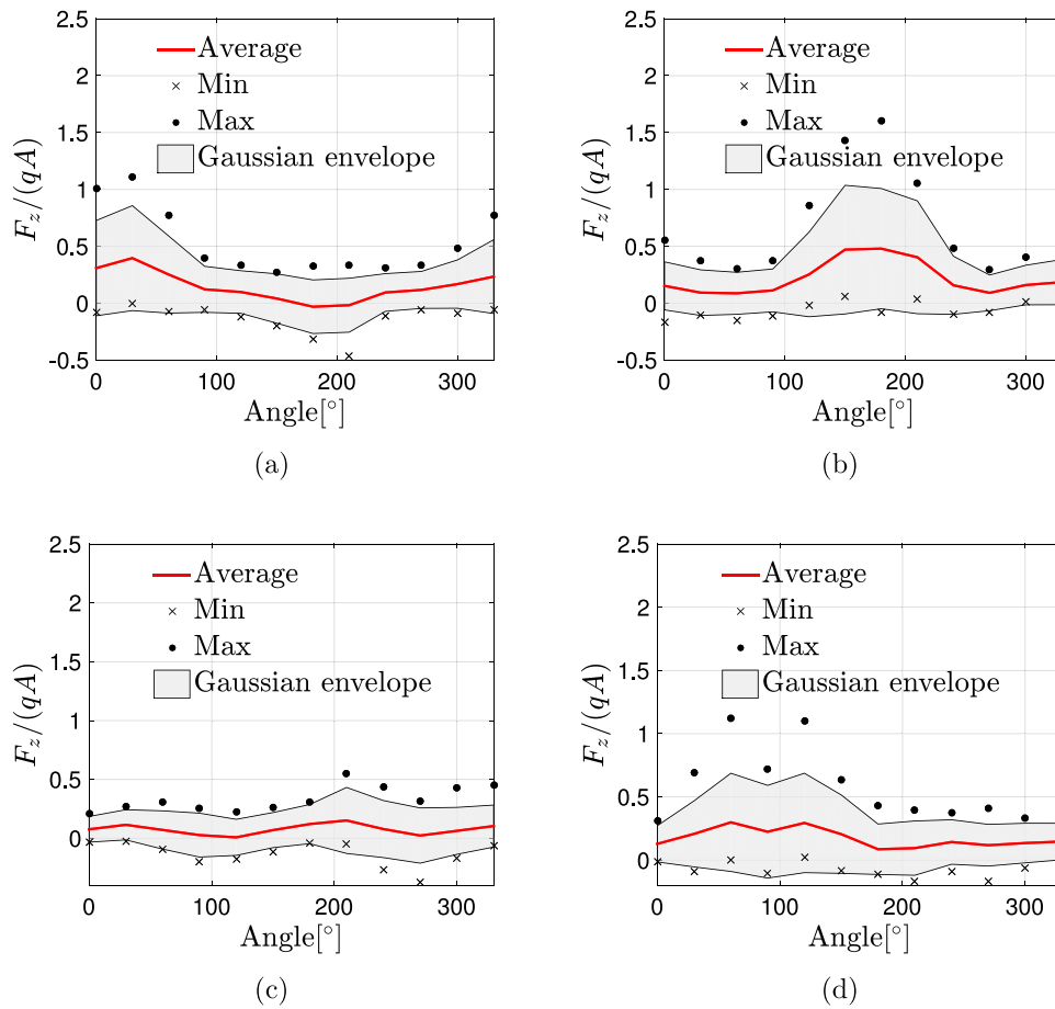
Fig. 12. Vertical force acting on each sector: (a) Sector 1, (b) Sector 2, (c) Sector 3 and (d) Sector 4. Forces are made non-dimensional with respect to the reference pressure, q = 0.5\rho U_r^2 , and the corresponding reference area, A .
