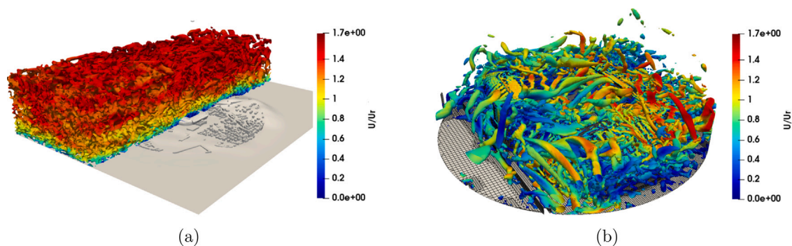
Fig. 7. Overview of the flow field by means of instantaneous Q-criterion iso-surfaces coloured by U/U_r : (a) overall domain ( Q = 0 ) and (b) around the stadium at 120^\circ ( Q = 2 ).
