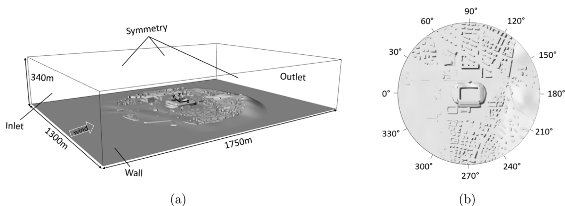
Fig. 2. The computational domain: (a) overview and (b) the rotor with indication of wind attack angles.
