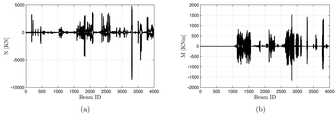
Fig. 22. Design envelopes for all structural members considering all wind directions: (a) axial forces and (b) bending moments.
